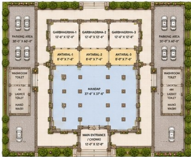
MASTER PLAN (PLOT SIZE 75'-0" X 75'-0")
