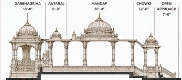
FRONT TO BACK SECTION (DEPTH 75'-0")
