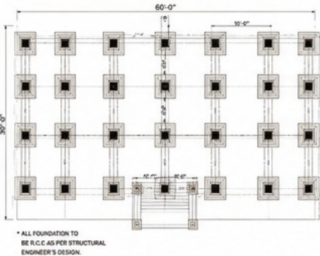
1. FOUNDATION PLAN
