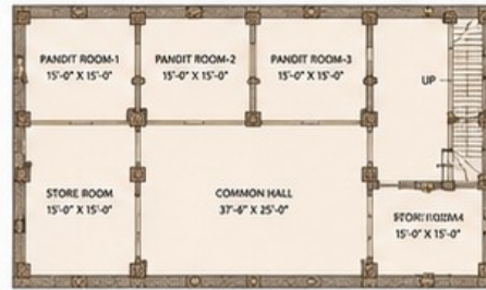
BASEMENT PLAN (FULL UNDER TEMPLE AREA)
